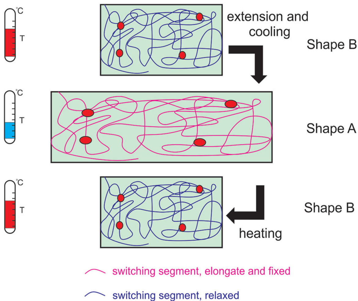
Figure 6. Molecular mechanism of temperature-responsive SMHs. The left panels represent the T_T related to the switching of conformational structure. The right panel represents the conformational change of the SMH from shape B to shape A upon cooling, and back from shape A to shape B upon application of heat. The covalent chemical bonds are represented by the red dots and the physical non-covalent bonds by the entangled lines. Reproduced with permission. [222] Copyright 2013, American Chemical Society.
